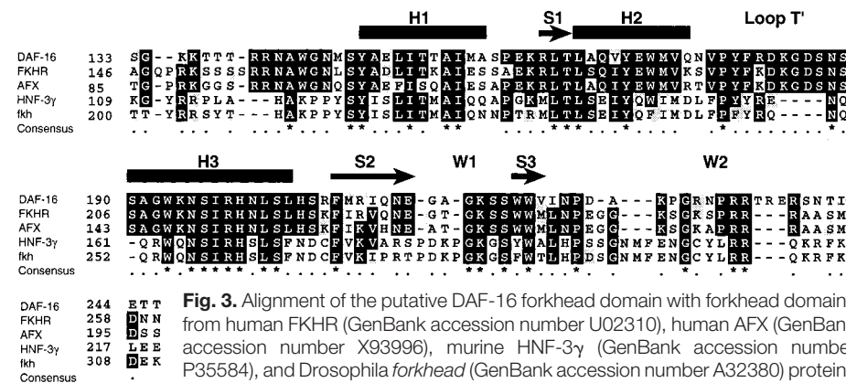
Fig. 3. Alignment of the putative DAF-16 forkhead domain with forkhead domains from human FKHR (GenBank accession number U02310), human AFX (GenBank accession number X93996), murine HNF-3γ (GenBank accession number P35584), and Drosophila forkhead (GenBank accession number A32380) proteins (20). Positions of the α helices (H1, H2, and H3), β strands (S1, S2, and S3), and wing (W1 and W2) domains as determined by x-ray crystallography of the HNF-3γ DNA binding domain (35) are indicated. Residues with greater than 50% identity and similarity are shaded in black and gray, respectively. Asterisks refer to residues that are identical in all five proteins; dots refer to residues that are similar in more than three of the proteins.
